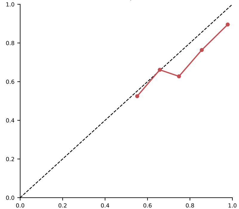
Unusable ECE=0.079, n=1957
