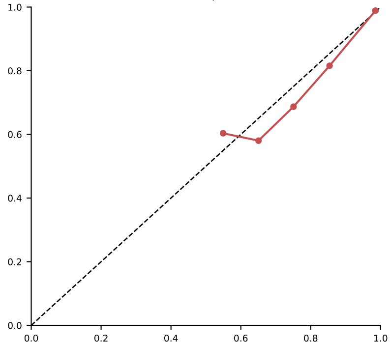
Usable ECE=0.010, n=7969
